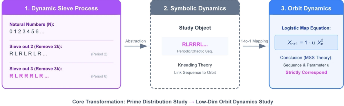
Figure 1. Core research framework for the Prime–Chaos problem. The diagram illustrates the theoretical pathway from the arithmetic sieve to symbolic sequences, which are subsequently mapped to the deterministic orbits of the Logistic chaotic attractor.
