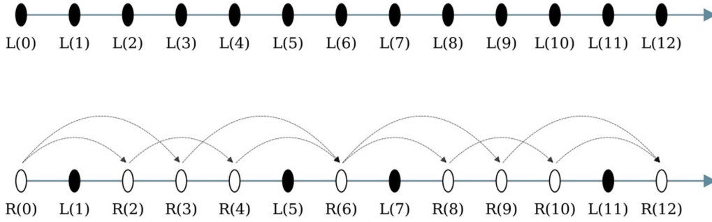
Figure 2. Example diagram of sieve composition rules, illustrating the dynamic sieving process on the natural number sequence starting from index 0.
