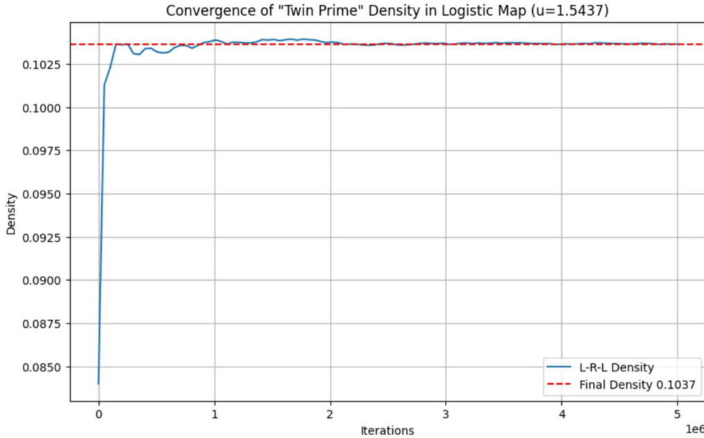
Figure 8. Numerical estimation of the intrinsic invariant measure ( \mu_{LRL} ). This figure illustrates the convergence of the cumulative probability of the orbit visiting the symbolic pattern L - R - L (Twin Prime cylinder set) in the standard autonomous Logistic map. Experimental Setup: The control parameter is fixed at the band-merging critical point u = u_c \approx 1.543689 , with a total simulation length of N = 10^9 . Results: The blue solid line represents the dynamic probability \mu(N) . As shown, the probability stabilises at the specific value \mu \approx 0.1037 (Red Dashed Line). Physical Significance: This value represents the intrinsic geometric measure of the ‘twin prime’ region in the attractor. It serves as the critical input for deriving the coupling constant k = 2C_2/\mu_{LRL} \approx 12.73 , ensuring the subsequent aging simulation is strictly parameter-free.
