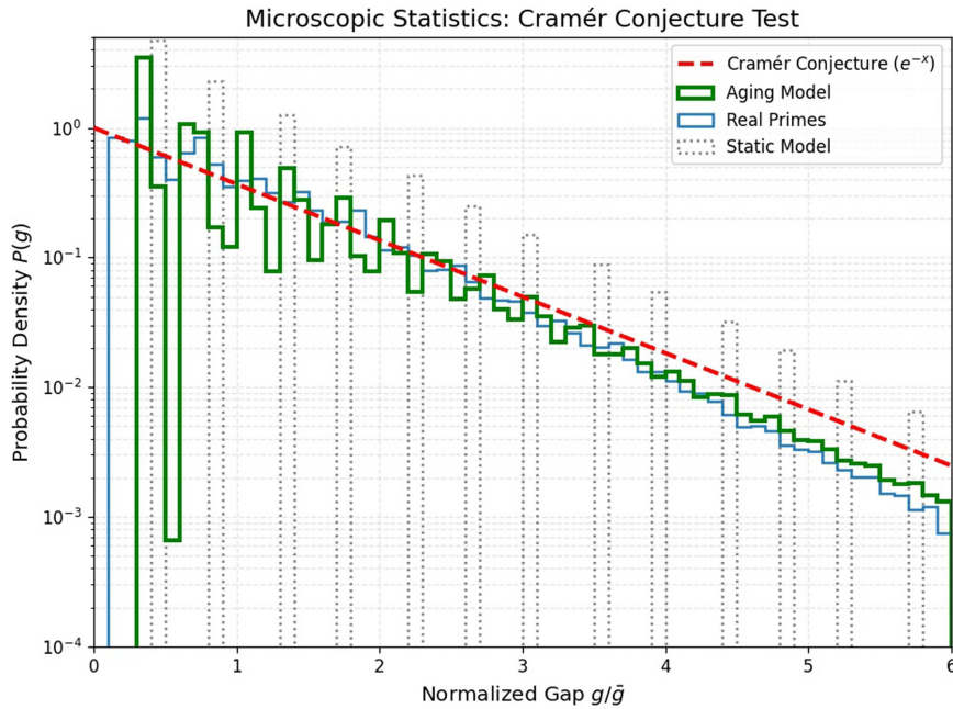
Figure 10. Microscopic statistics: test of the Cramér conjecture. The figure compares the probability density of normalised gaps g/\bar{g} against the exponential distribution predicted by the Cramér conjecture (Red Dashed Line, e^{-x} ). Key Result: While the Static Model (Grey Dotted Line) deviates significantly from the theoretical curve, the Aging Model (Green Solid Line) perfectly collapses onto the exponential curve, exhibiting statistical behaviour indistinguishable from Real Primes (Blue Solid Line).
