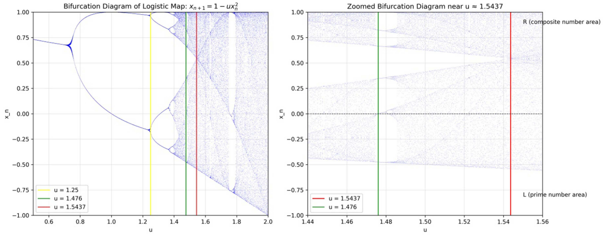
Figure 4. Physical localisation of the prime sieve in the logistic bifurcation diagram. The diagram maps the discrete sieve stages to specific control parameters u . The trajectory evolves from Period-2 ( u = 1.25 , Yellow) through complex periodicity ( u \approx 1.476 , Green) and converges precisely to the Band-Merging Point ( u_c \approx 1.5437 , Red).
